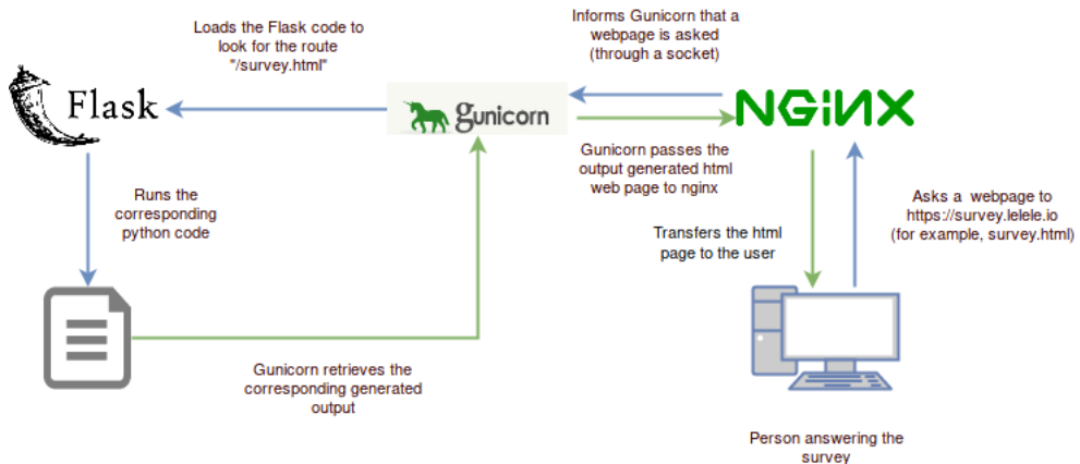
Figure 3.5: nginx/Gunicorn/Flask workflow
