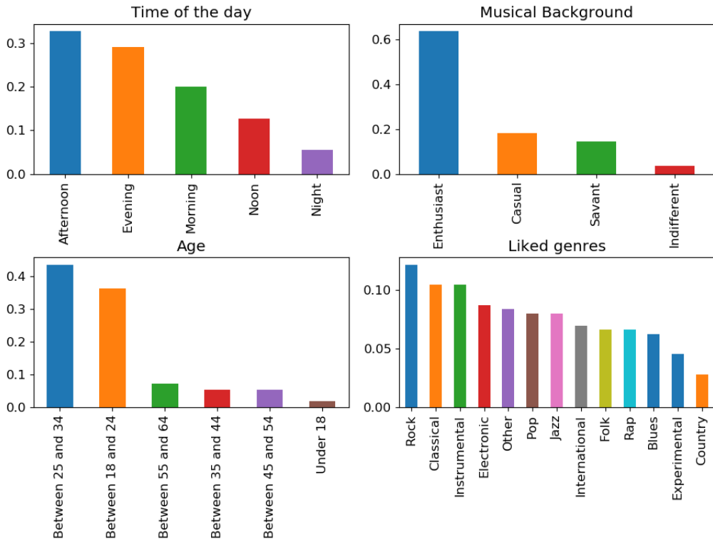
Figure 3.7: Demographics results
